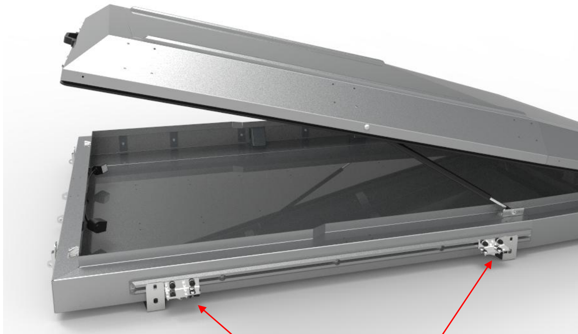
Spring pole cargo rail brackets installed. LHS bracket on the left & and RHS Bracket on the right
